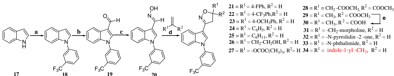
Figure 3. Synthesis of compounds 18–34 . Reagents and conditions: (a) 1-bromo-3-(trifluoromethyl) benzene, \text{Cs}_2\text{CO}_3 , CuI, DMF, 165^\circ\text{C} , 3–4 h, 77%; (b) \text{POCl}_3 , DMF, 165^\circ\text{C} , 2–3 h, 75%; (c) \text{NH}_2\text{OH}\cdot\text{HCl}/\text{C}_5\text{H}_5\text{N}/\text{C}_2\text{H}_5\text{OH} , rt, 15–16 h, 90%; (d) different alkenes/THF, bleach, rt, 24–26 h, 10–90%; (e) compound 30 from 29 , THF/MeOH/ \text{H}_2\text{O} , LiOH, rt, 3 h, 78%.
