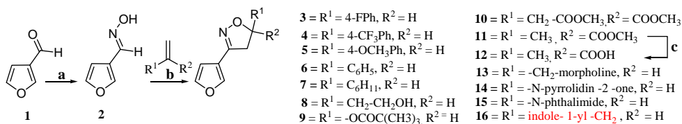
Figure 2. Synthesis of compounds 2–16 . Reagents and conditions: (a) \text{NH}_2\text{OH}\cdot\text{HCl}/\text{C}_5\text{H}_5\text{N}/\text{C}_2\text{H}_5\text{OH} , rt, 15–16 h, 90%; (b) different alkenes/THF, bleach, rt, 24–26 h, 10–90%; (c) compound 12 from 11 , THF/MeOH/ \text{H}_2\text{O} , LiOH, rt, 3 h, 82%.
